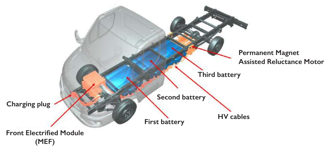
Example of an eDaily 3 modular batteries
