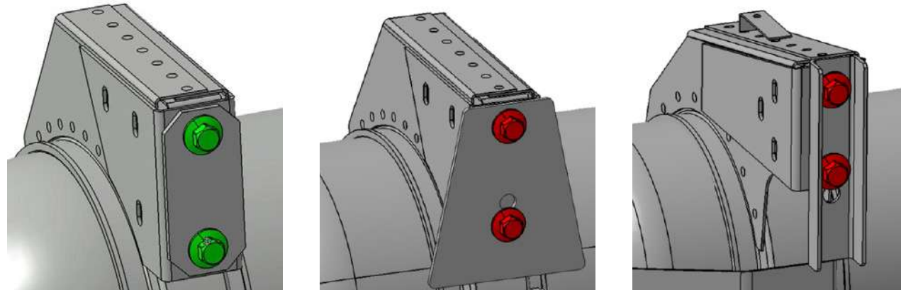
Tank support brackets to chassis and rear cross member fastening with stiffening plates
